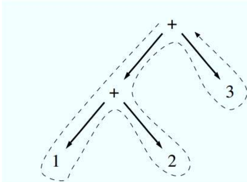
Depth first tree walk path: node discovery, finishing
