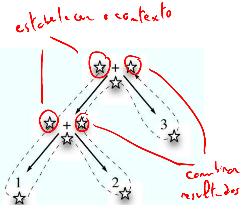
Traversal order: action execution opportunities
